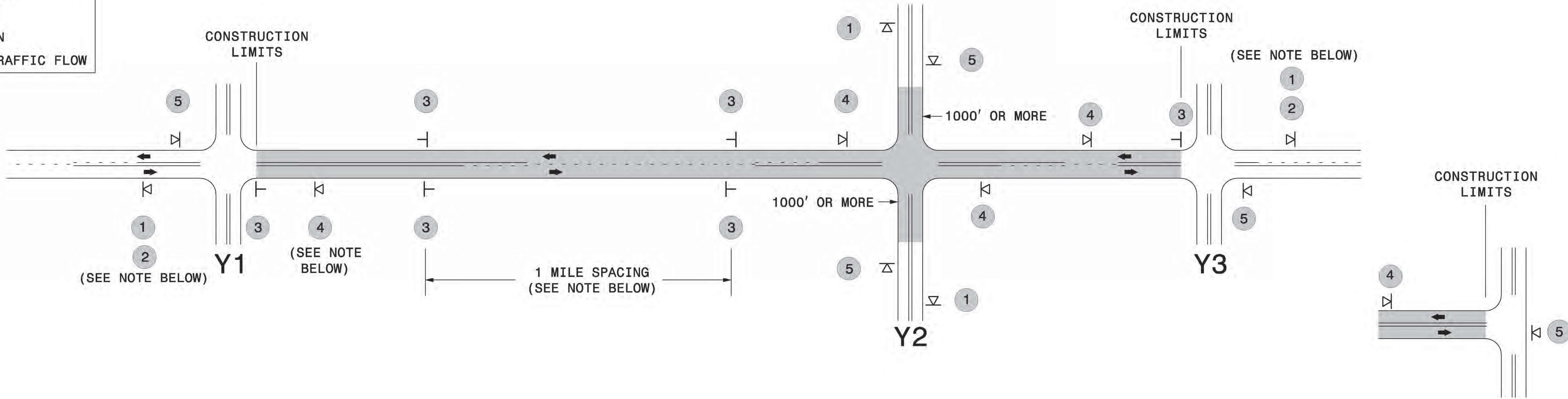
TEE INTERSECTION
